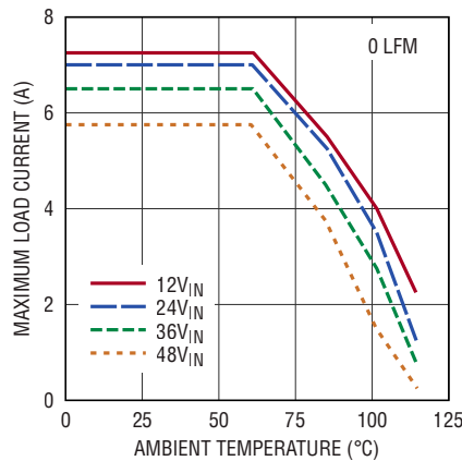
Derating, V_{OUT} = 3.3\text{V} , BIAS = 5V, DC2387A Demo Board
